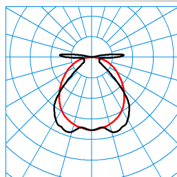
AragF 15 P-W 80-840 PC HT TX371729
